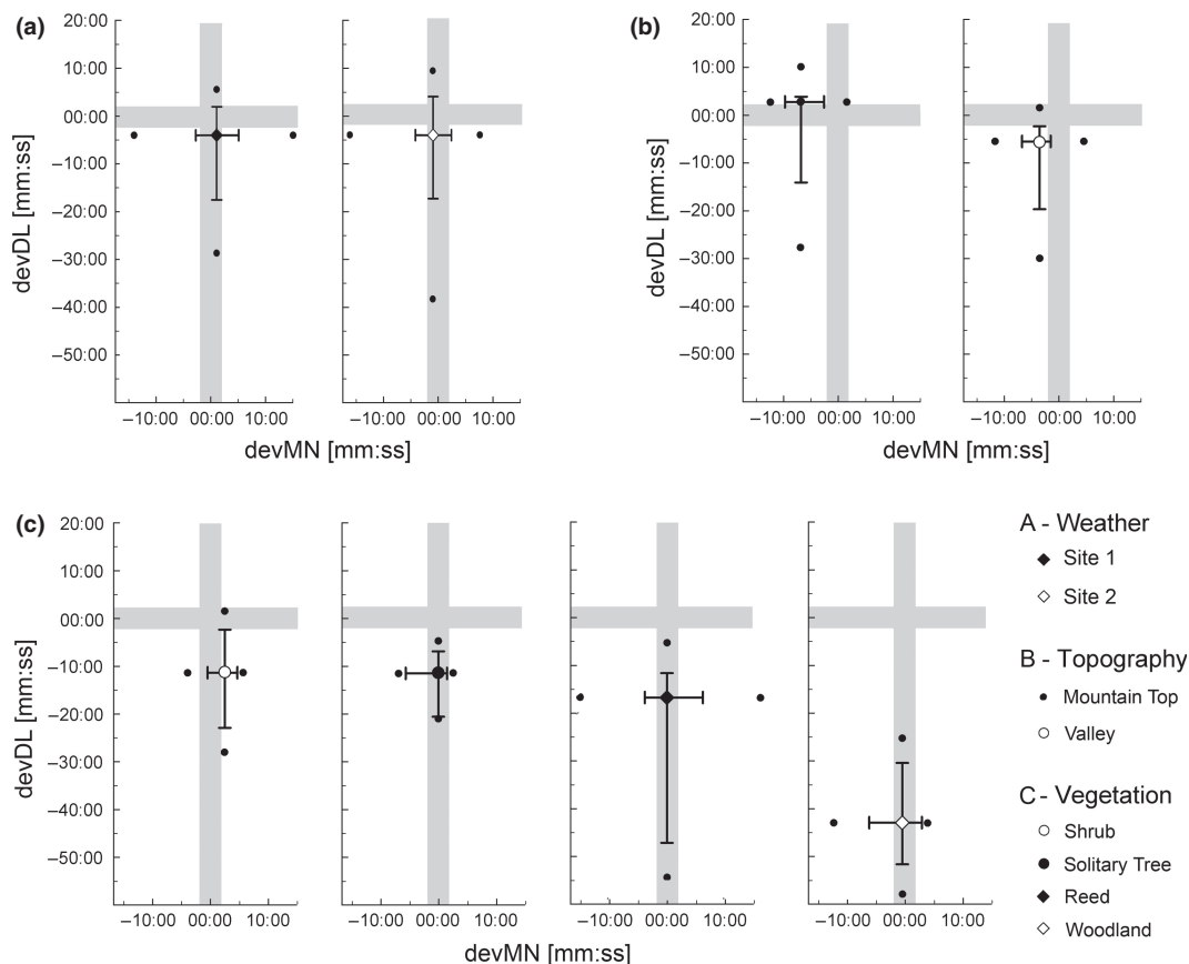
Fig. 3. Deviation from 'true' day length (devDL) and solar midnight/noon (devMN) in mins of stationary geolocators which were exposed to the effects of (a) weather, (b) topography plus weather and (c) vegetation plus weather. For deviations, mode values and 10 and 90 percentile values are given; extremes are symbolized as dots. The grey bars indicate the range of \pm 2 min, which is the potential highest accuracy of each sunrise and sunset time determined by refraction at the horizon.
