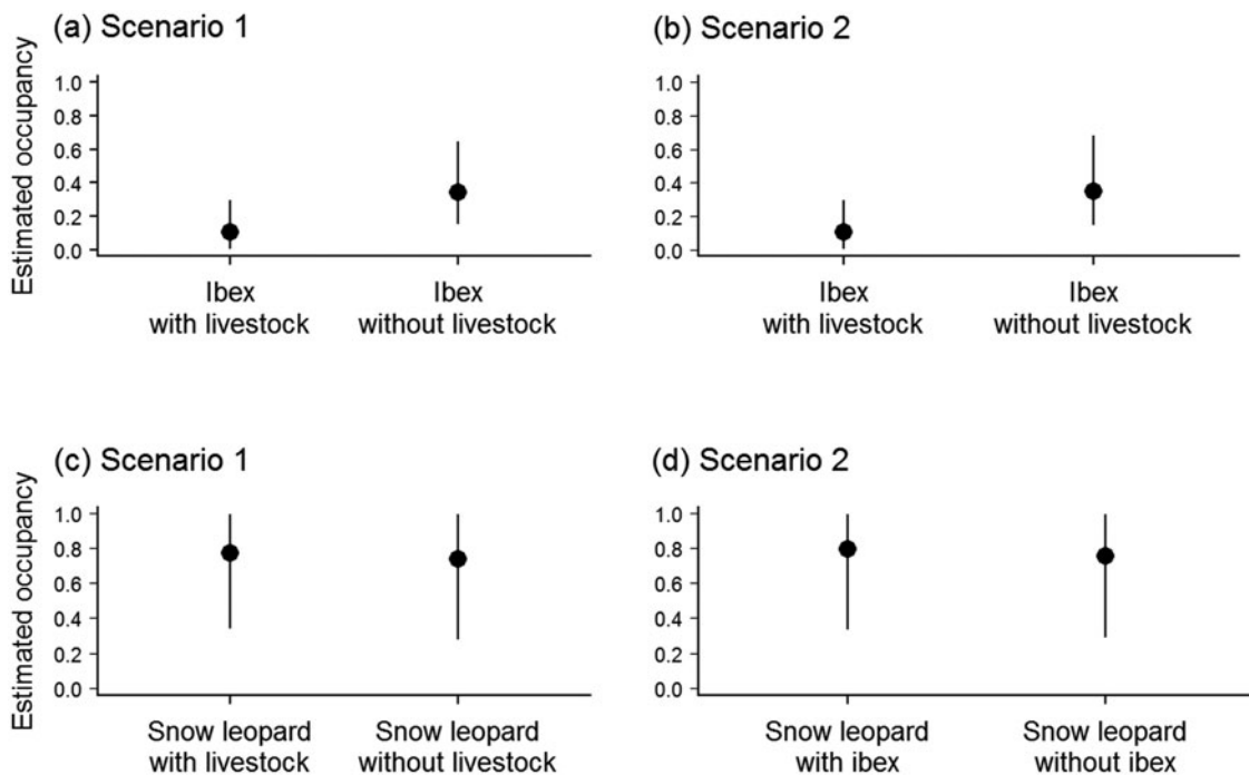
FIG. 2 Occupancy probability (mean and 95% credible interval) estimated from the modelling of co-occurrence patterns of (a) ibex depending on livestock, scenario 1; (b) ibex depending on livestock, scenario 2; (c) snow leopard depending on livestock, scenario 1; and (d) snow leopard depending on ibex, scenario 2.
