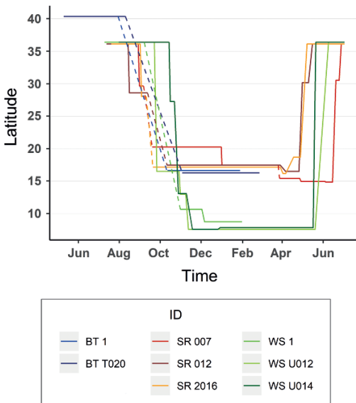
FIG. 2.—Latitude crossings ( ^{\circ} N) from breeding to winter grounds and back of White-rumped Swifts ( N = 3 , green colours), Rufous-tailed Scrub-robins ( N = 3 , red, brown and orange colours) and Bluethroats ( N = 2 , blue colours) with time (days). Data logging of one White-rumped Swift and the two Bluethroats stopped during winter. WS = White-rumped Swift, SR = Rufous-tailed Scrub-robin; BT = Bluethroat.
