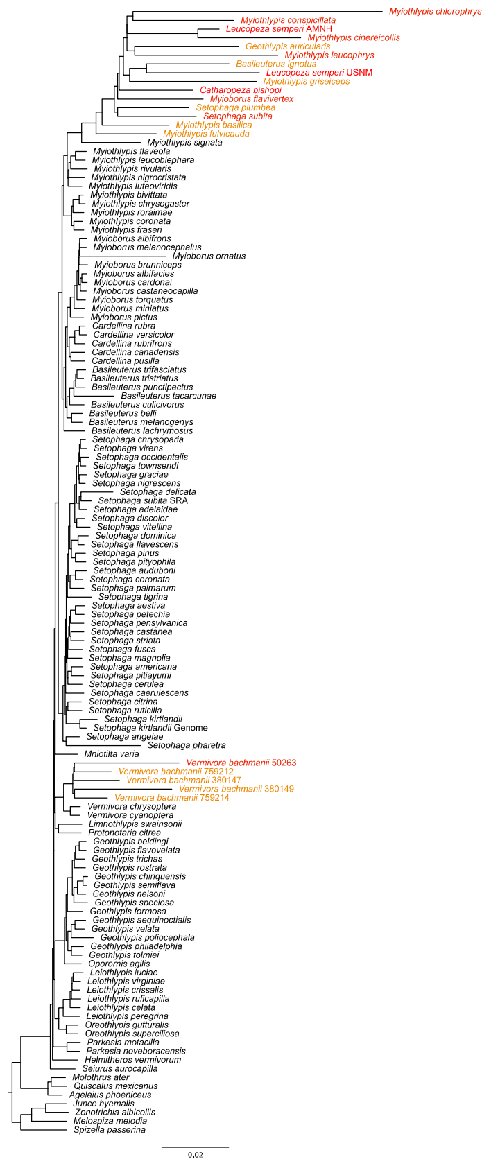
Fig. 1. Concatenated tree of 122 parulid samples based on the unfiltered UCE dataset, highlighting clustering of poorly performing samples. The phylogenetic positions for bad samples (tip labels in orange) and ugly samples (tip labels in red) appeared problematic (except for Vermivora bachmanni ) and were explored in additional analyses. (For interpretation of the references to color in this figure legend, the reader is referred to the web version of this article.)
